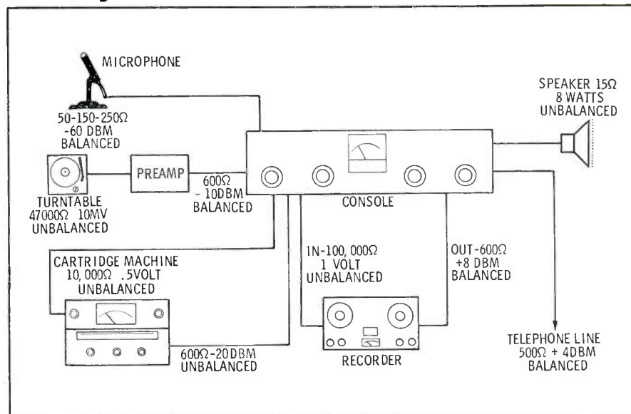
Fig. 4. Typical levels and impedances encountered during sound recording work.
