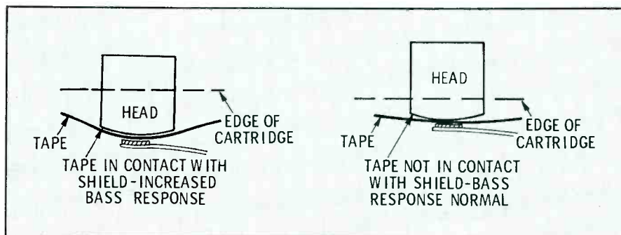
Fig. 3. Relative position of both tape and head affects bass response of the machine.
